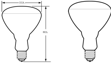
GE Reveal BR30
